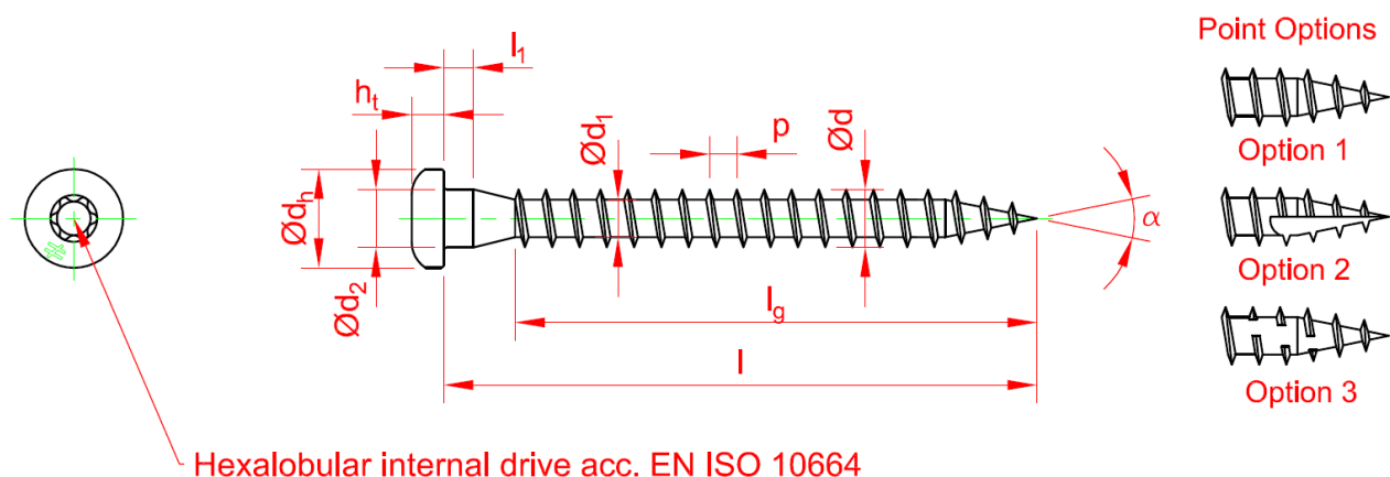
Drawing 2: CSA Connector screw
