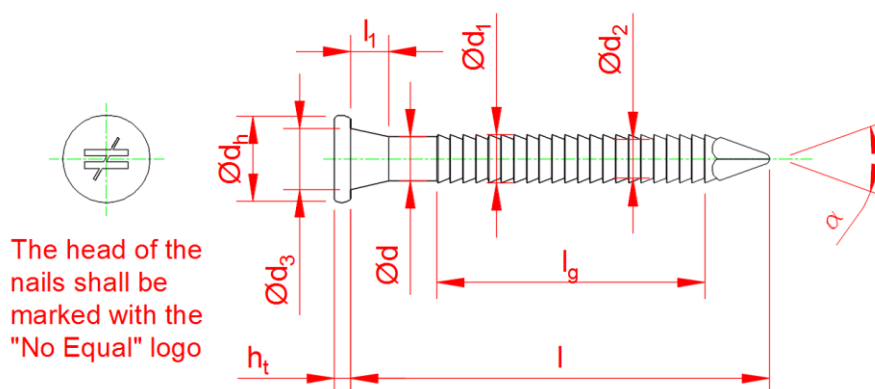
Drawing 1: CNA Connector nails
